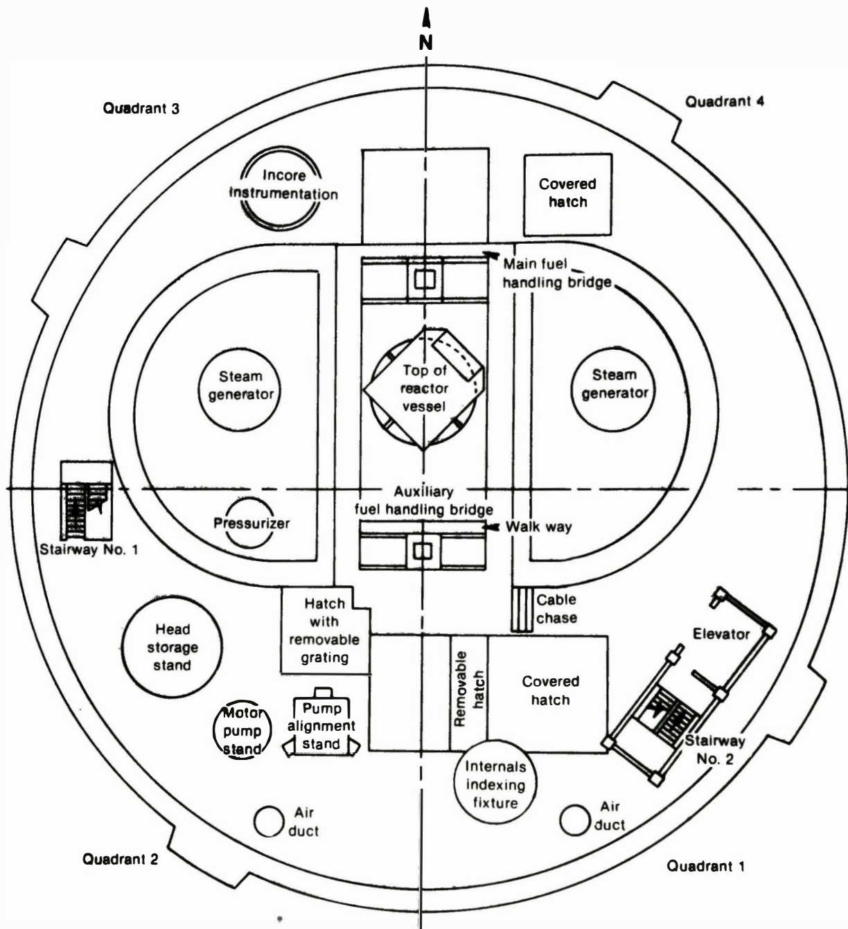
Figure 5. Elevation 347 diagram.
