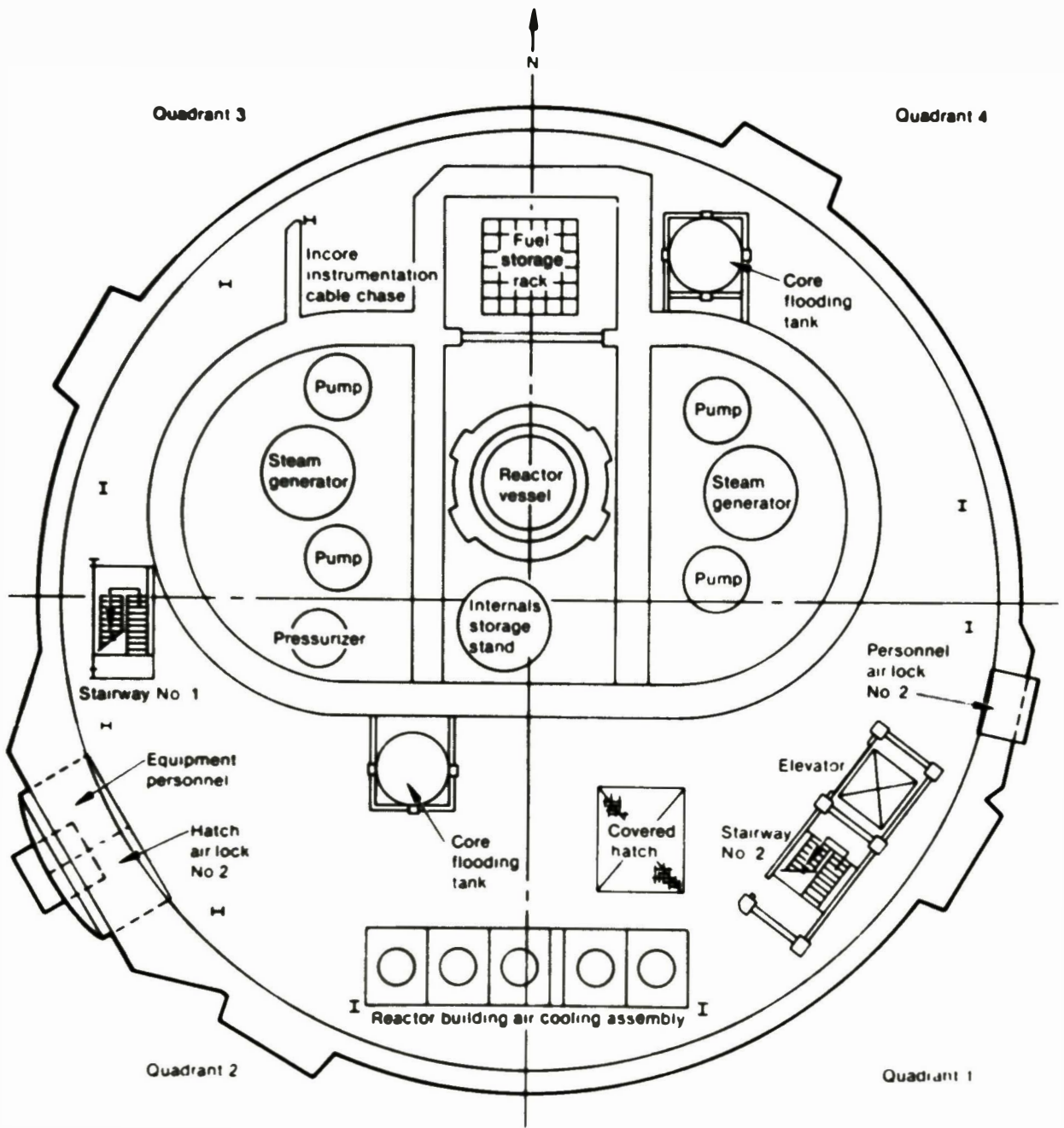
Figure 1. Elevation 305 diagram.
